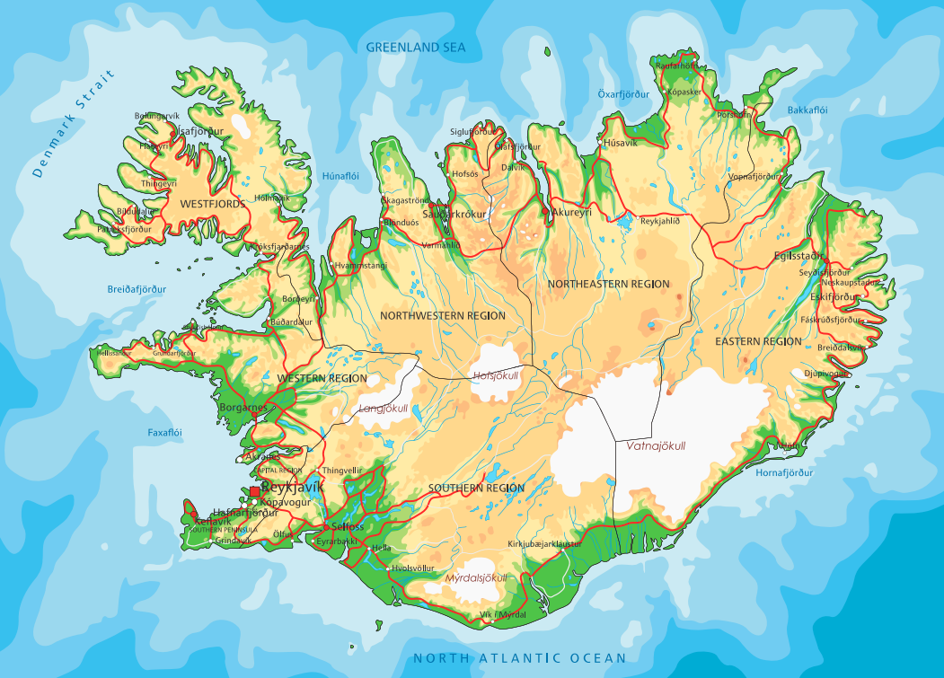
GEYSIR
